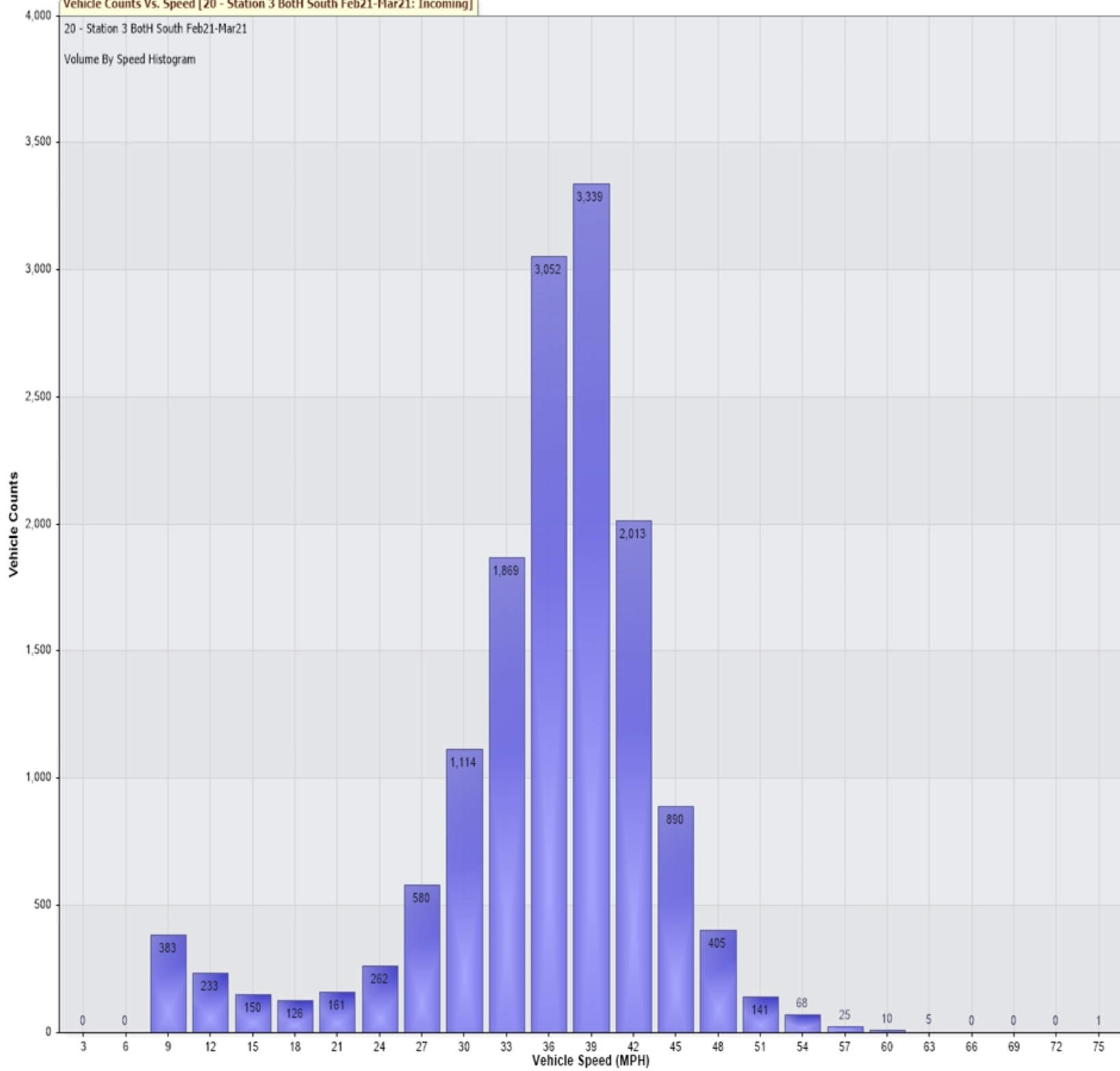
Vehicle Counts Vs. Speed [20 - Station 3 Both South Feb21-Mar21: Incoming]
