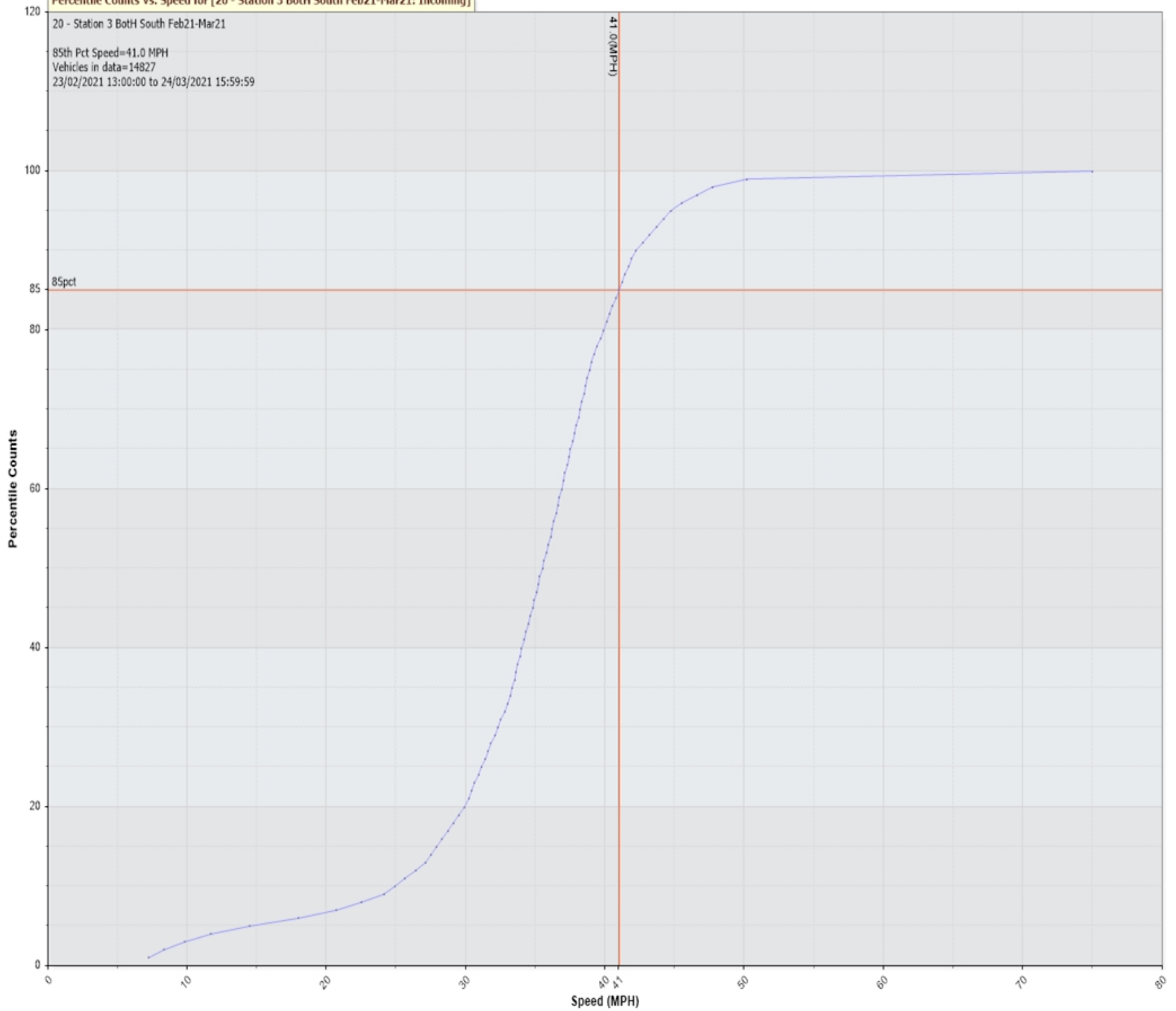
Percentile Counts Vs. Speed for [20 - Station 3 Both South Feb21-Mar21: Incoming]
