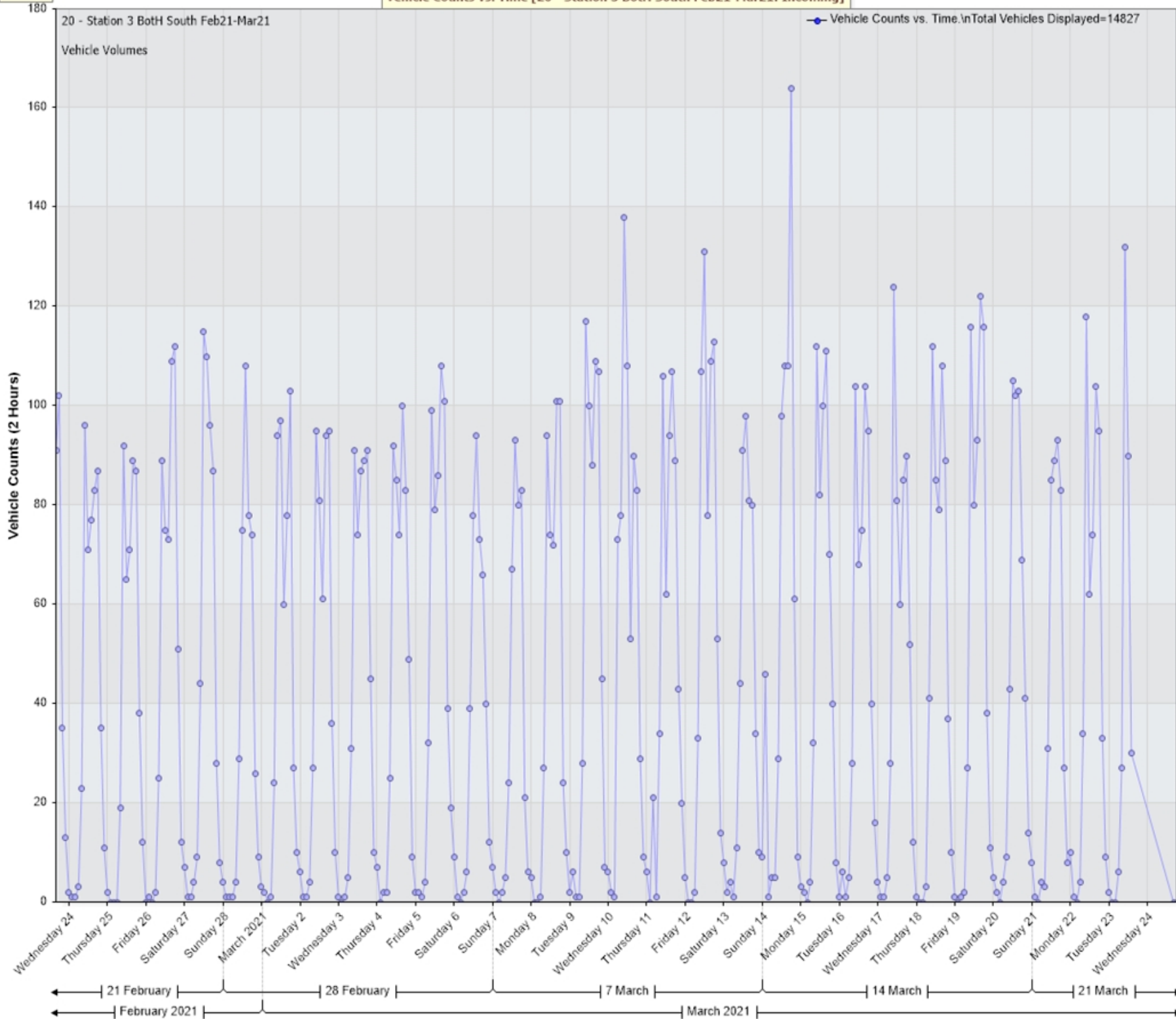
Vehicle Counts vs. Time [20 - Station 3 Both South Feb21-Mar21: Incoming]
