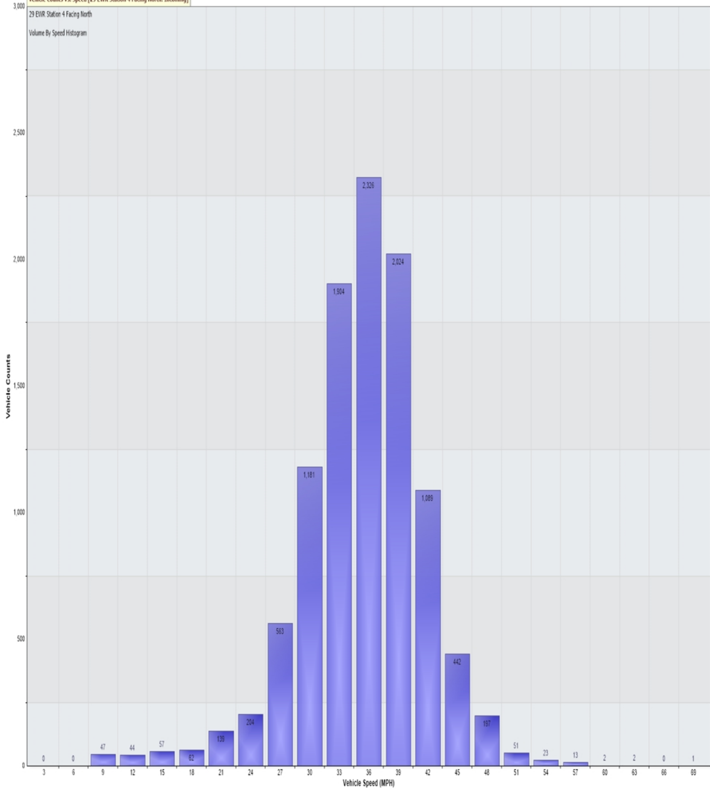
Vehicle Counts Vs. Speed [29 EWR Station 4 Facing North: Incoming]
