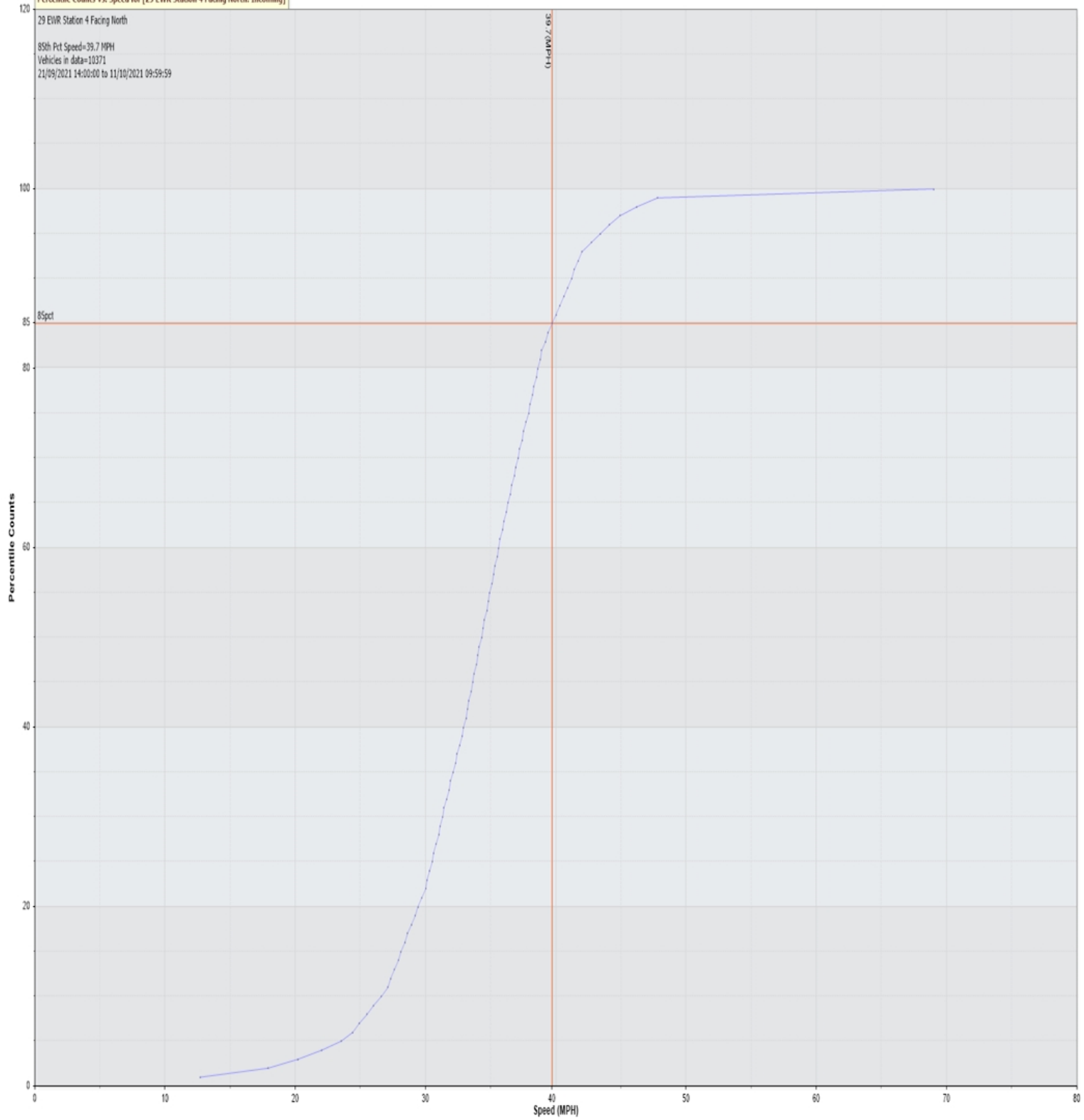
Percentile Counts Vs. Speed for [29 EWR Station 4 Facing North: Incoming]
