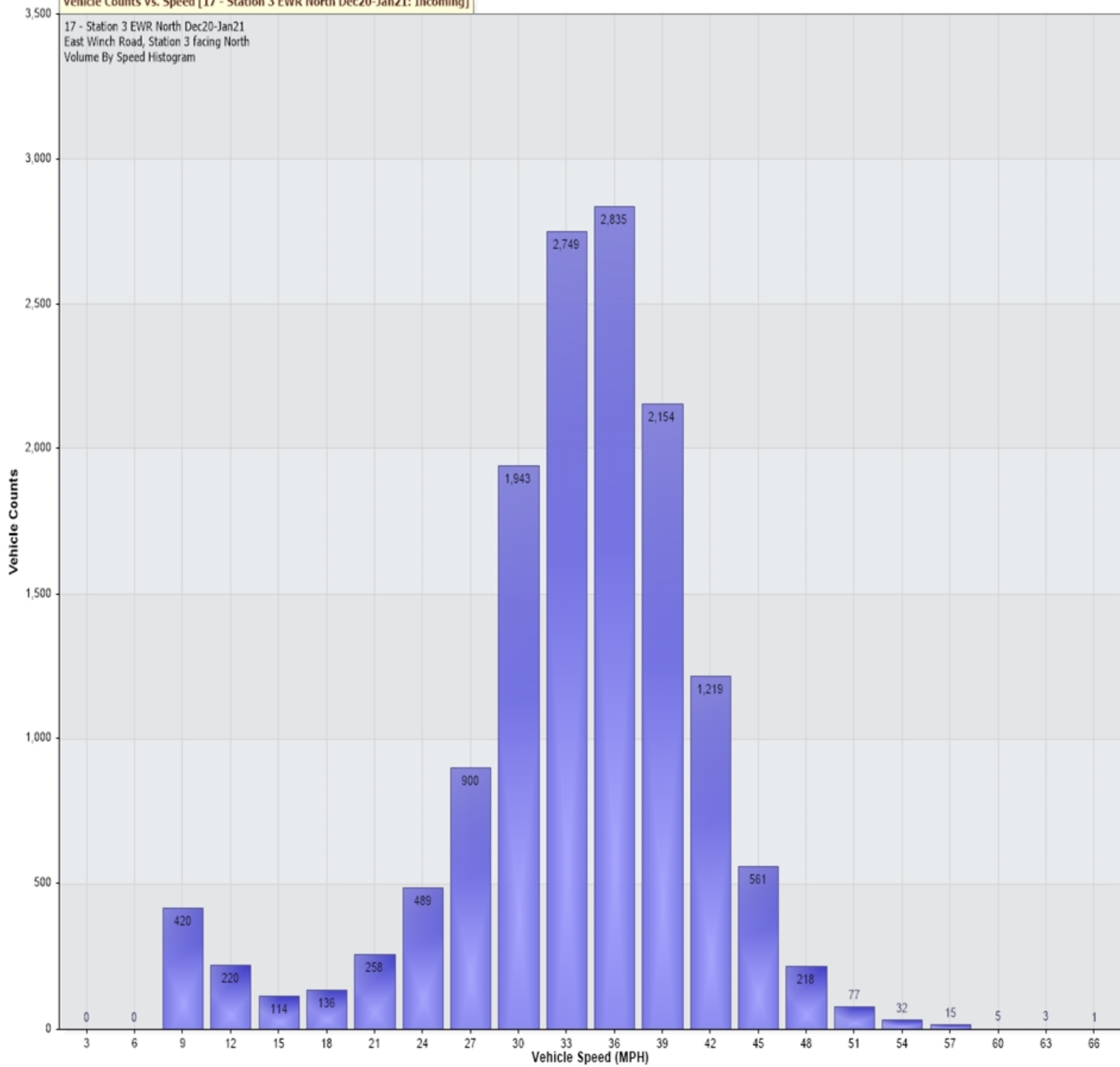
Vehicle Counts Vs. Speed [17 - Station 3 EWR North Dec20-Jan21: Incoming]
