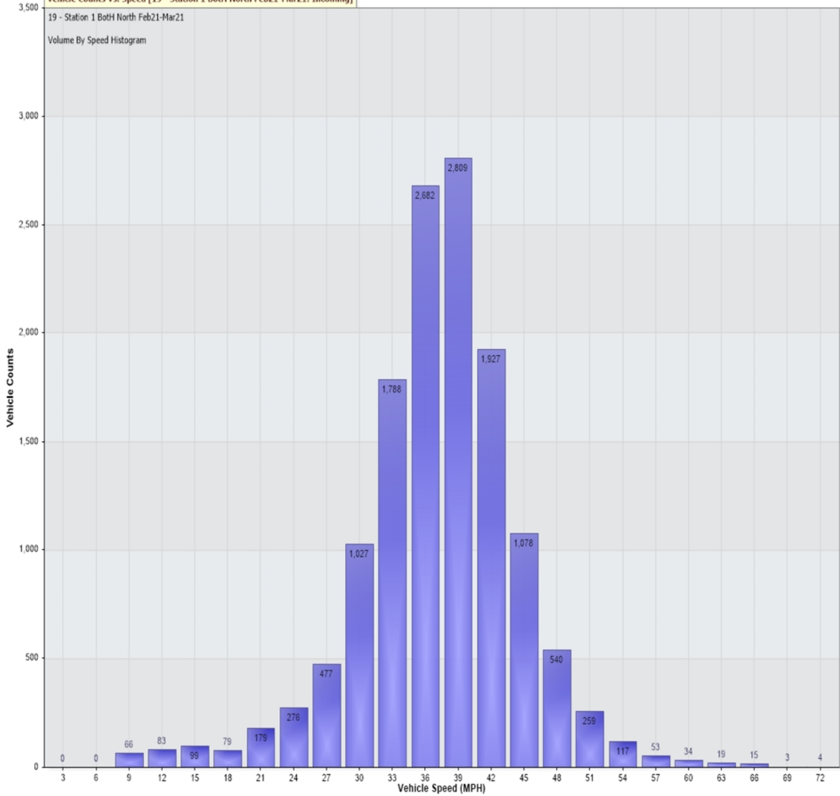
Vehicle Counts Vs. Speed [19 - Station 1 Both North Feb21-Mar21: Incoming]
