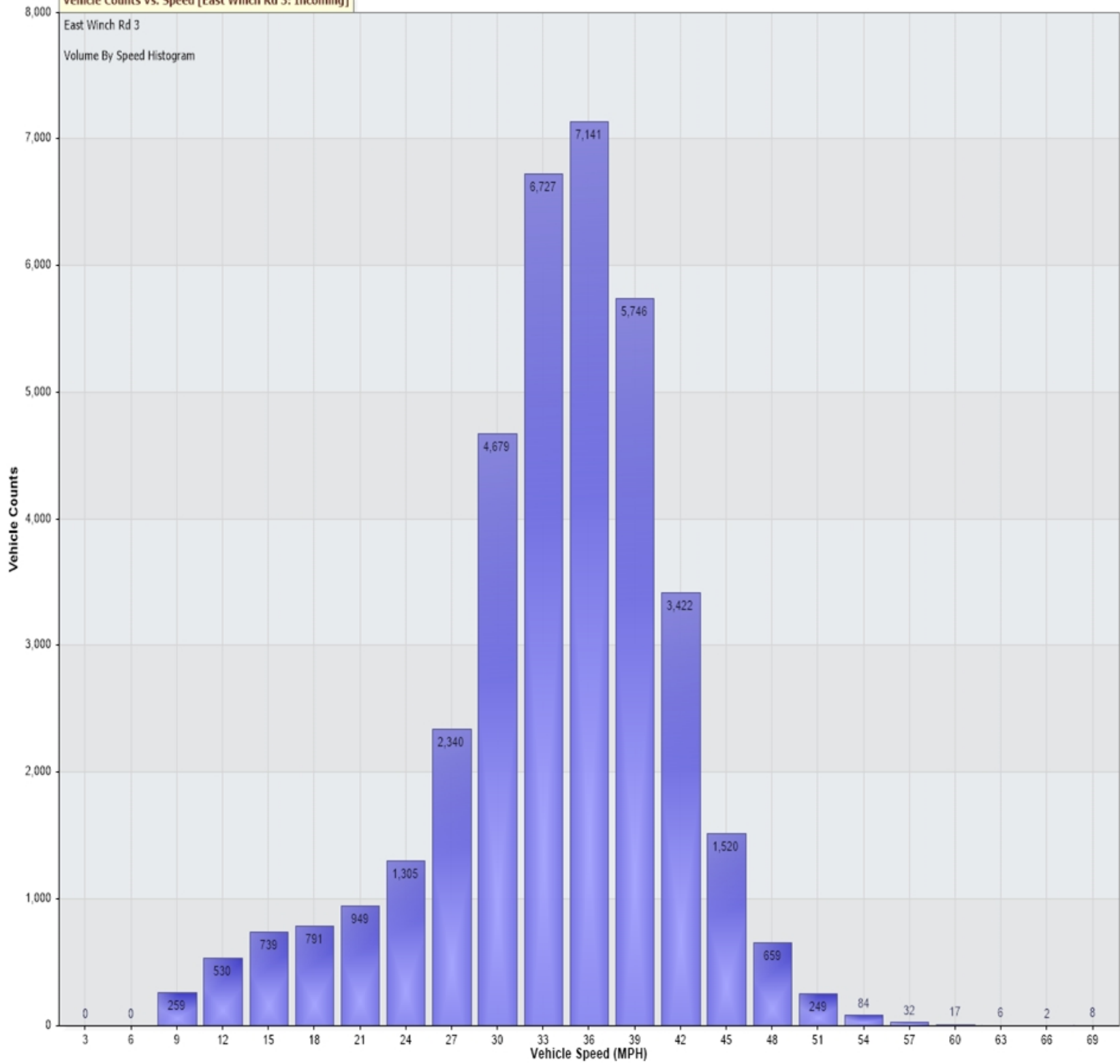
Vehicle Counts Vs. Speed [East Winch Rd 3: Incoming]
