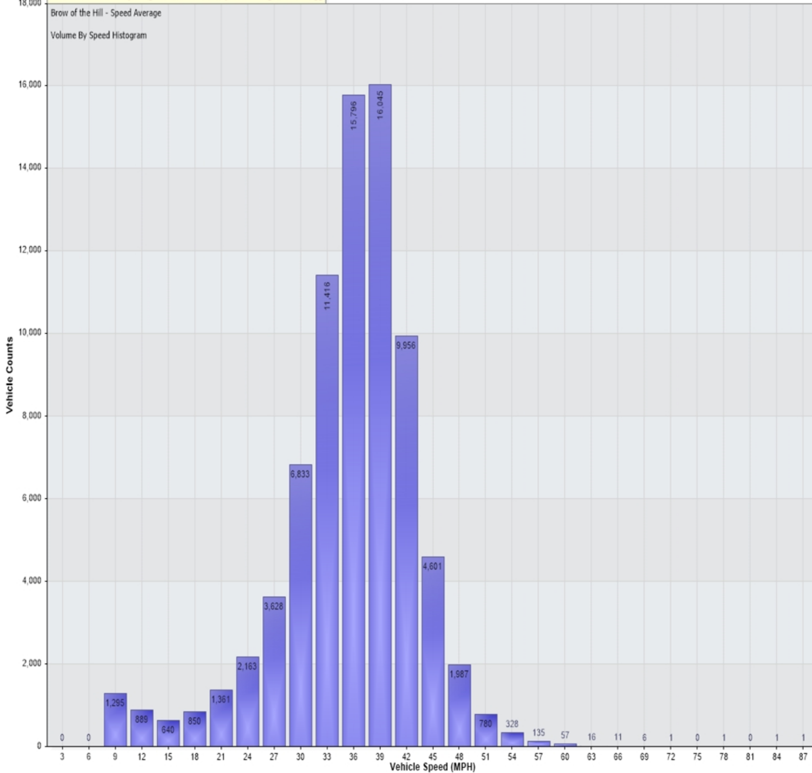
Vehicle Counts Vs. Speed [Brow of the Hill - Speed Average: Incoming]
