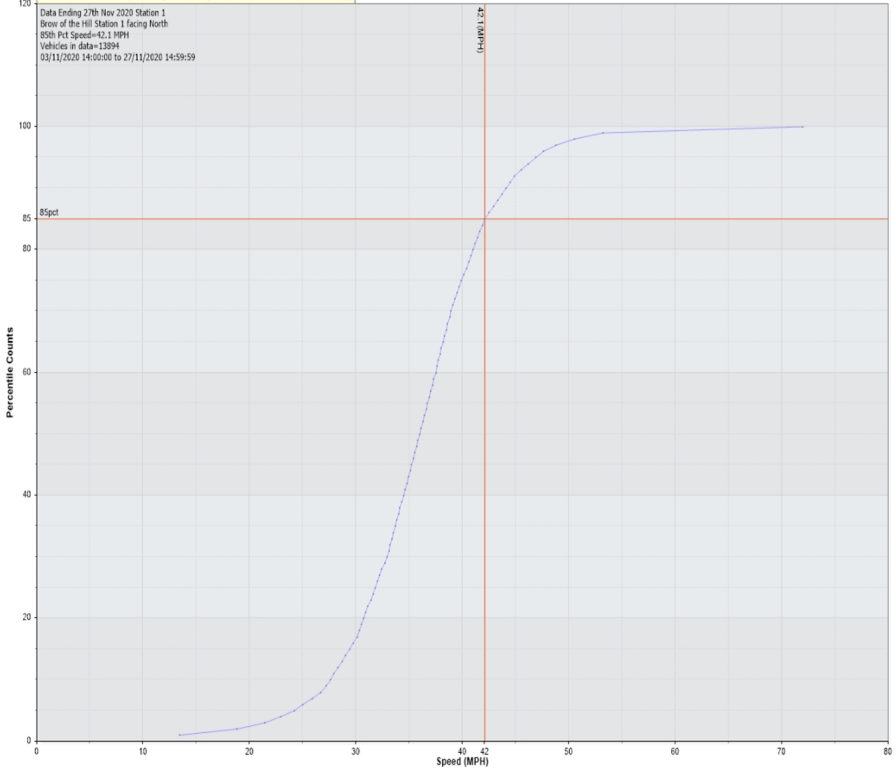
Percentile Counts Vs. Speed for [Data Ending 27th Nov 2020 Station 1: Incoming]
