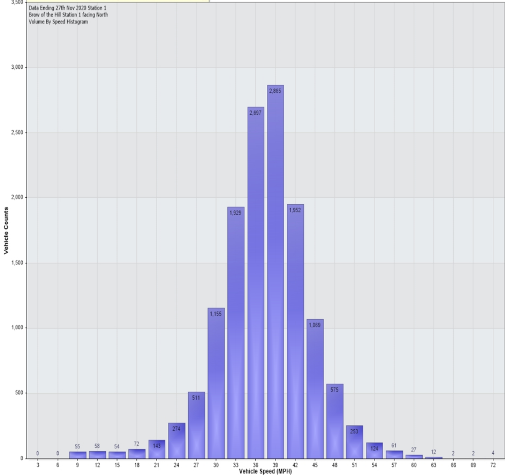
Vehicle Counts Vs. Speed [Data Ending 27th Nov 2020 Station 1: Incoming]
